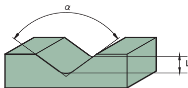
V-groove treatment for oil pressure parts Depth L control
