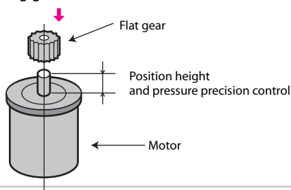
Attaching gear to motor
