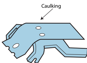
Caulking for attaching relay switch
